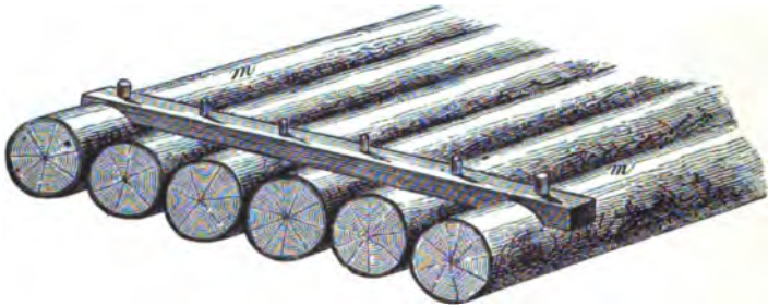
Fig 275.—Fixing a section by a plank.
